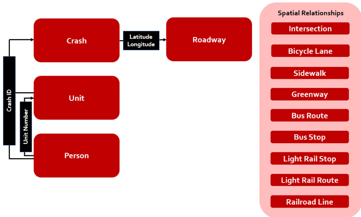
Figure 2. Charlotte HSIS Data Files and Linking Variables.
